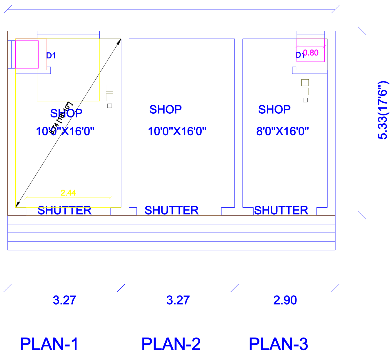
G.FLOOR PLAN
