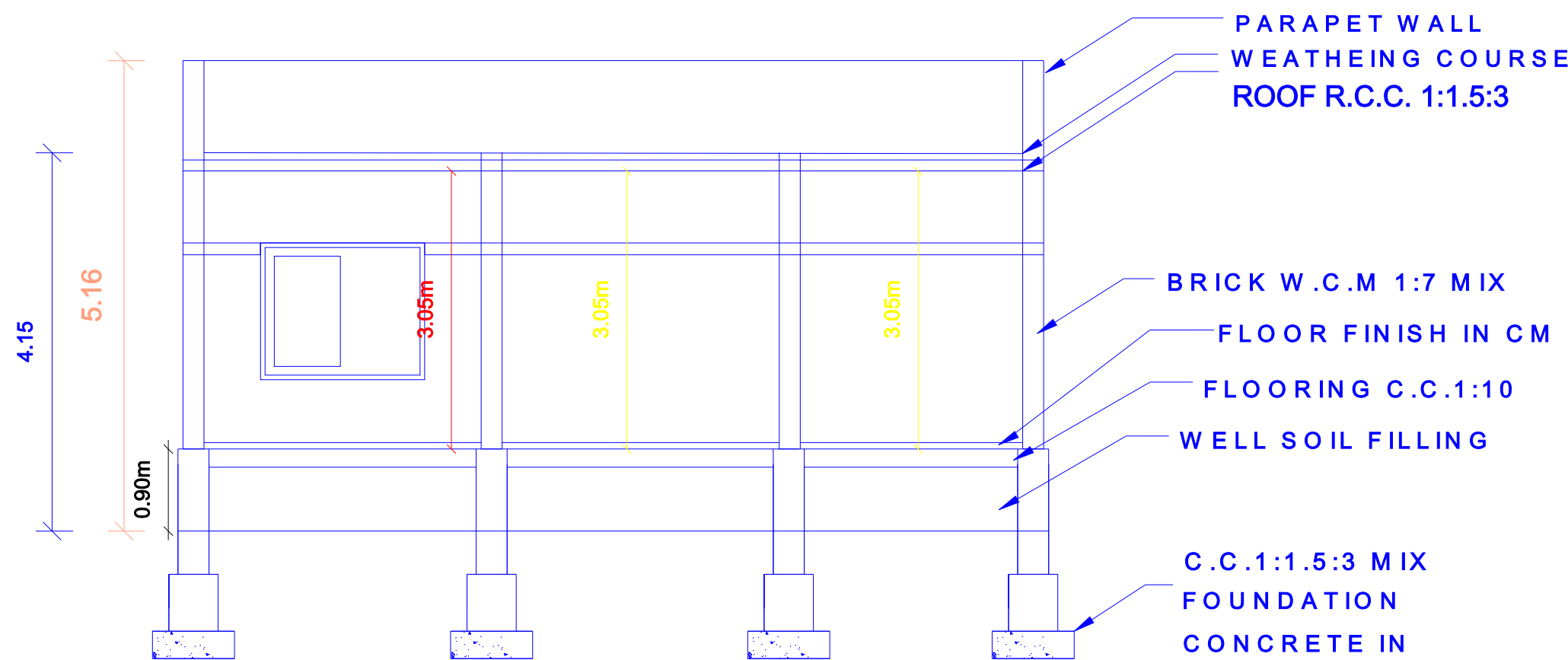
SECTION
