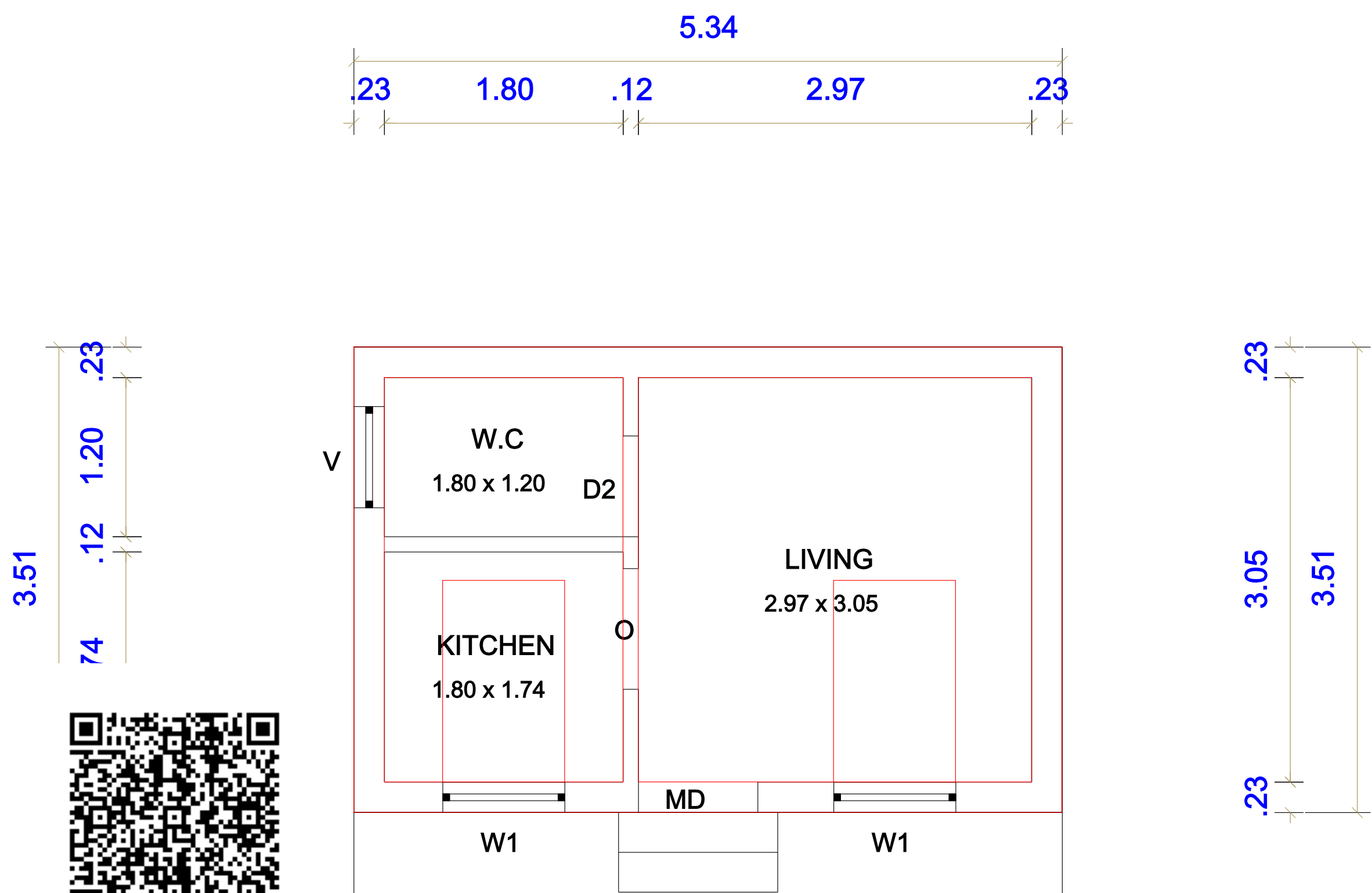
PLAN
