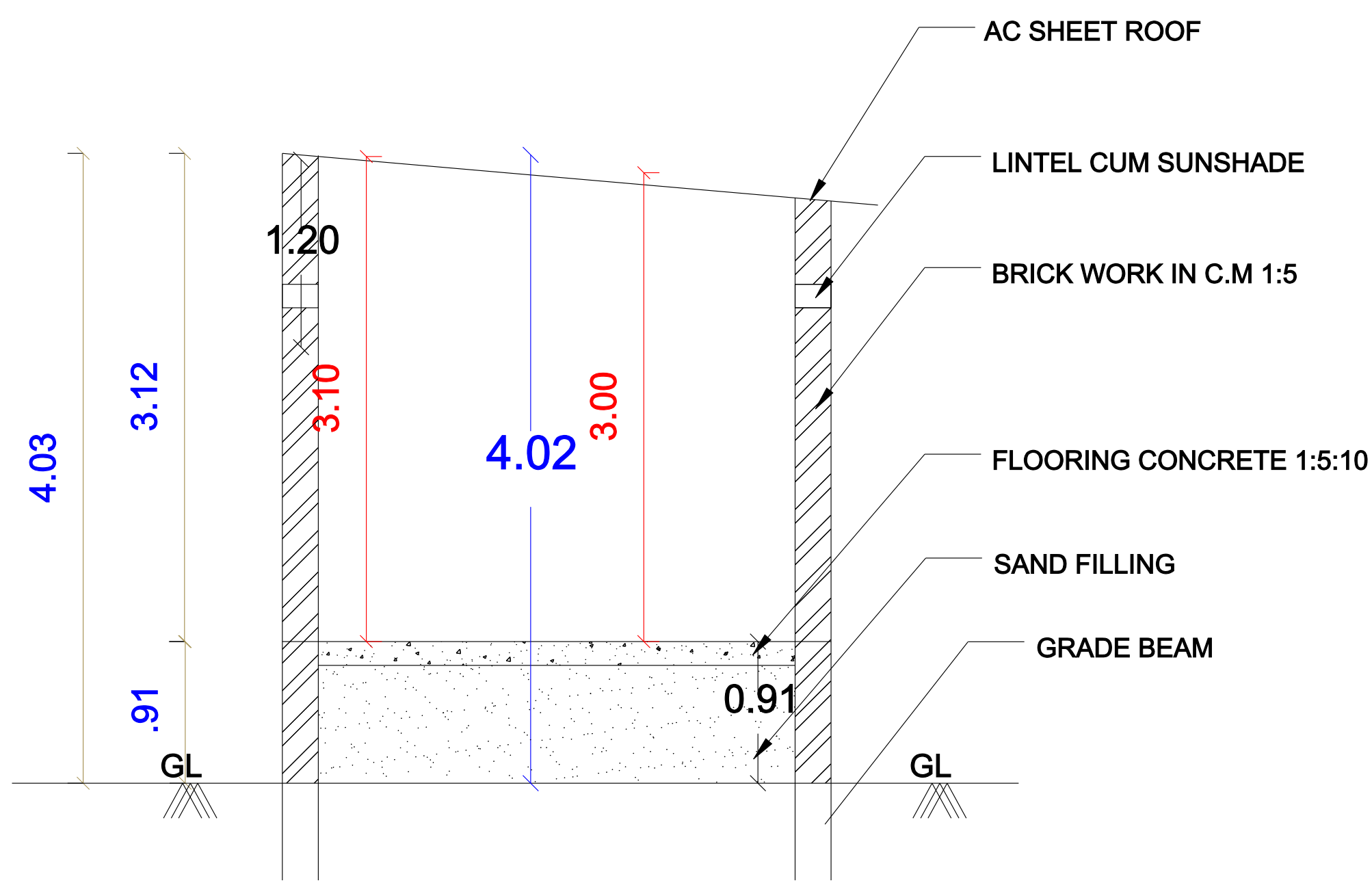
SECTION-"AA"
