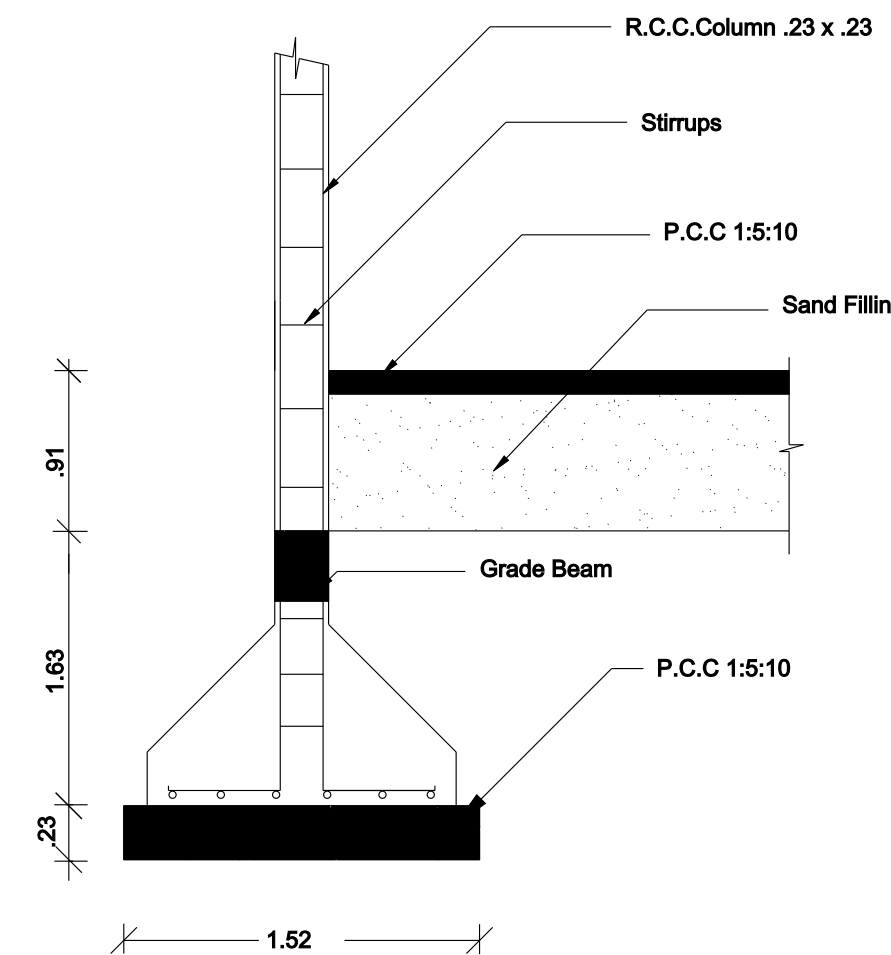
COLUMN DETAIL
