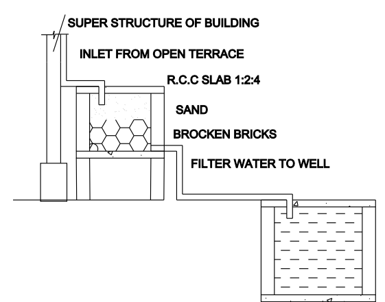
RAINWATER HARVESTING
