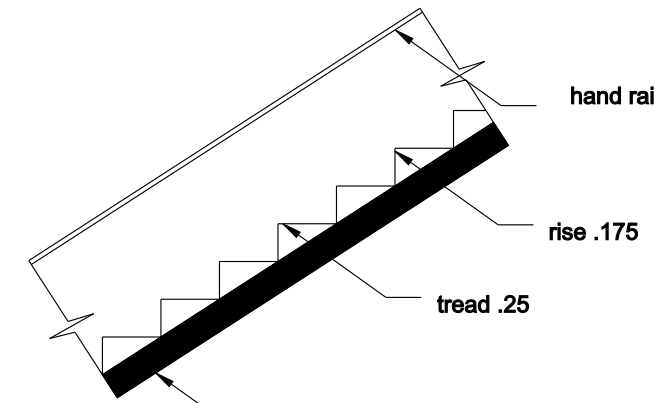
STAIR
