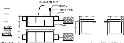
SEPTIC TANK AND TRENCH NTS
