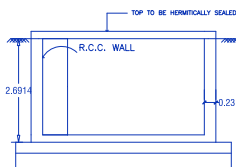
RWH_CAPACITY_L=5000LTRS RWH_CAPACITY_L=5000LTRS
