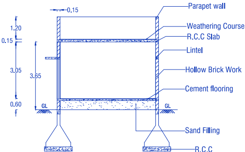
CROSS SECTION ON 'AB'
