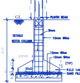
SECTION ON DWARF WALL (DW)
