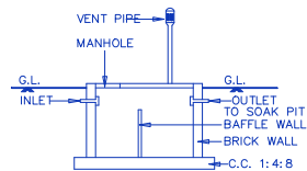
SECTION OF SEPTIC TANK
