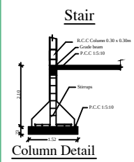
Column Detail
