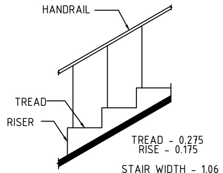
STAIRCASE DETAILS
