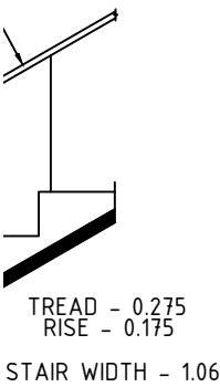
STAIRCASE DETAILS NTS
