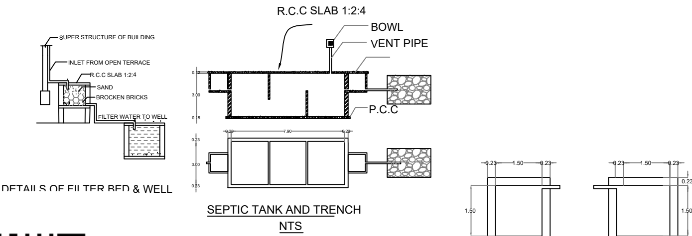
RAIN WATER HVESTING
