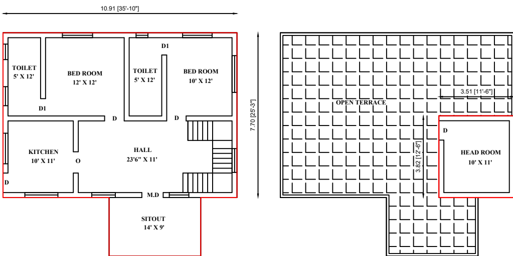
HEAD ROOM PLAN
