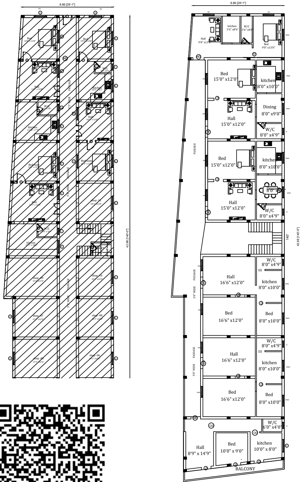
AN PRO FIRST FLOOR PLAN
