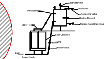
Details Of Solar Water Heater (NTS)
