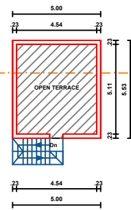
TERRACE PLAN
