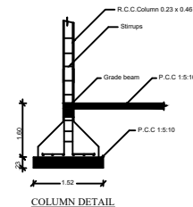
COLUMN DETAIL
