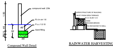
Compound Wall Detail
