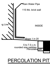
PERCOLATION PIT
