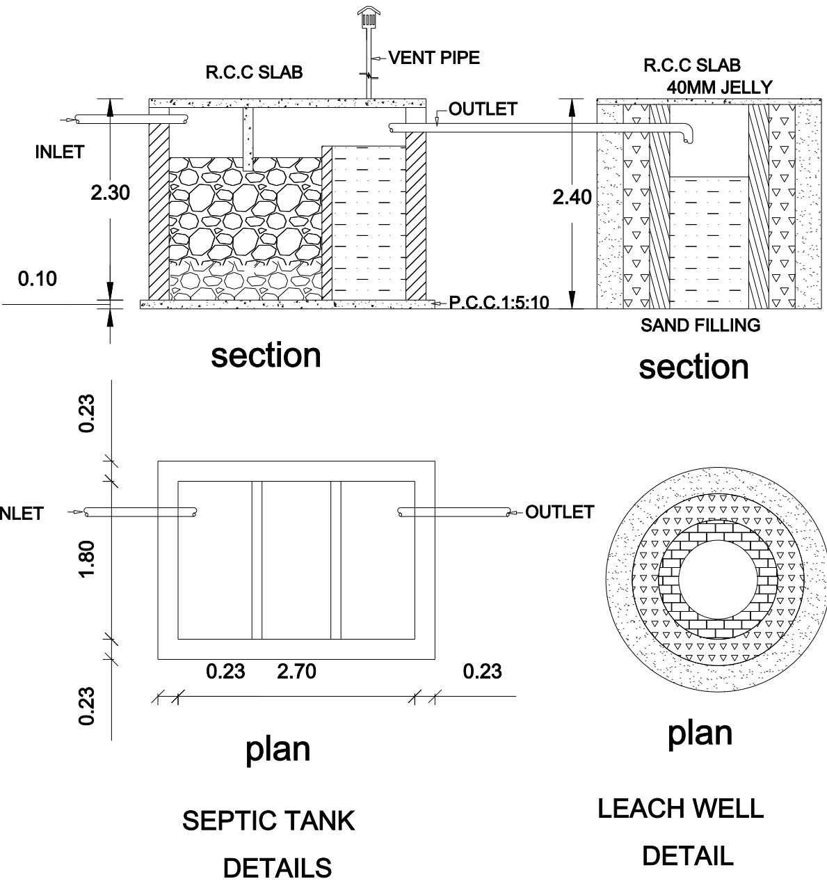
1000 GALLONS CAPACITY SEPTIC TANK ( NTS )
