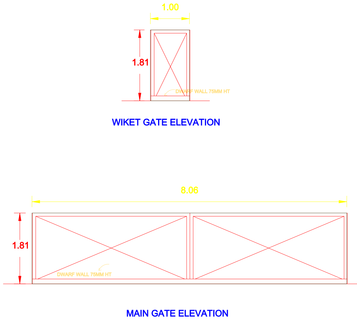
MAIN GATE ELEVATION
