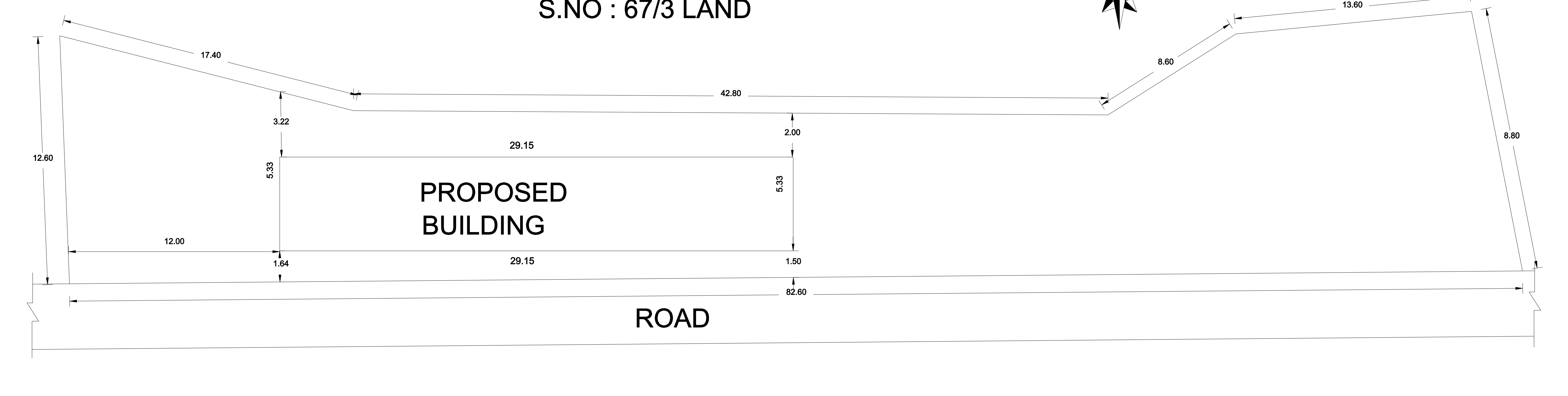
SITE PLAN ( SCALE:- 1:200 )
