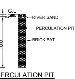
PERCULATION PIT
