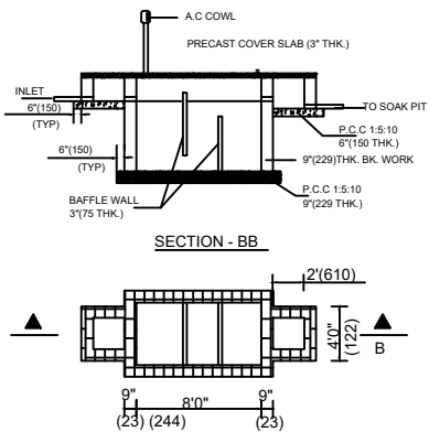
SECTION - BB
