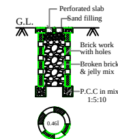
PERCOLATION PIT (NOT FOR SCALE)
