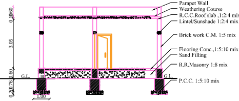
SECTION ON A-R
