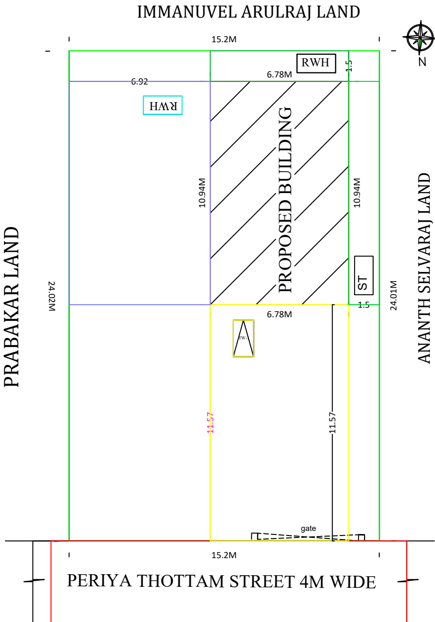
KEY PLAN 1:100 SCALE
