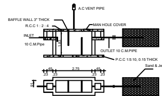
SEPTIC TANK AND TRENCH
