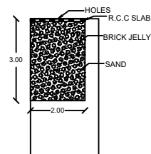
SECTION OF RAIN WATER COLLECTING TANK
