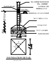
FOUNDATION DETAIL
