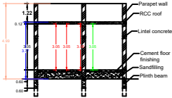
SECTION - "AB"
