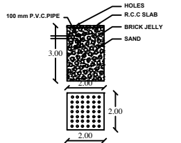
RAIN WATER COLLECTING TANK
