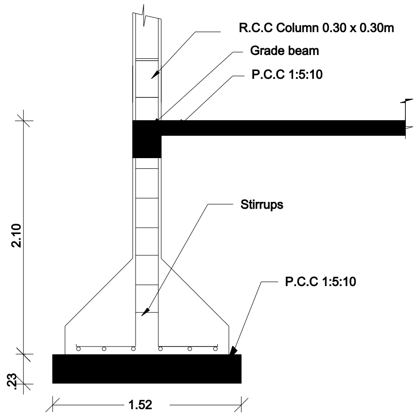
Column Detail
