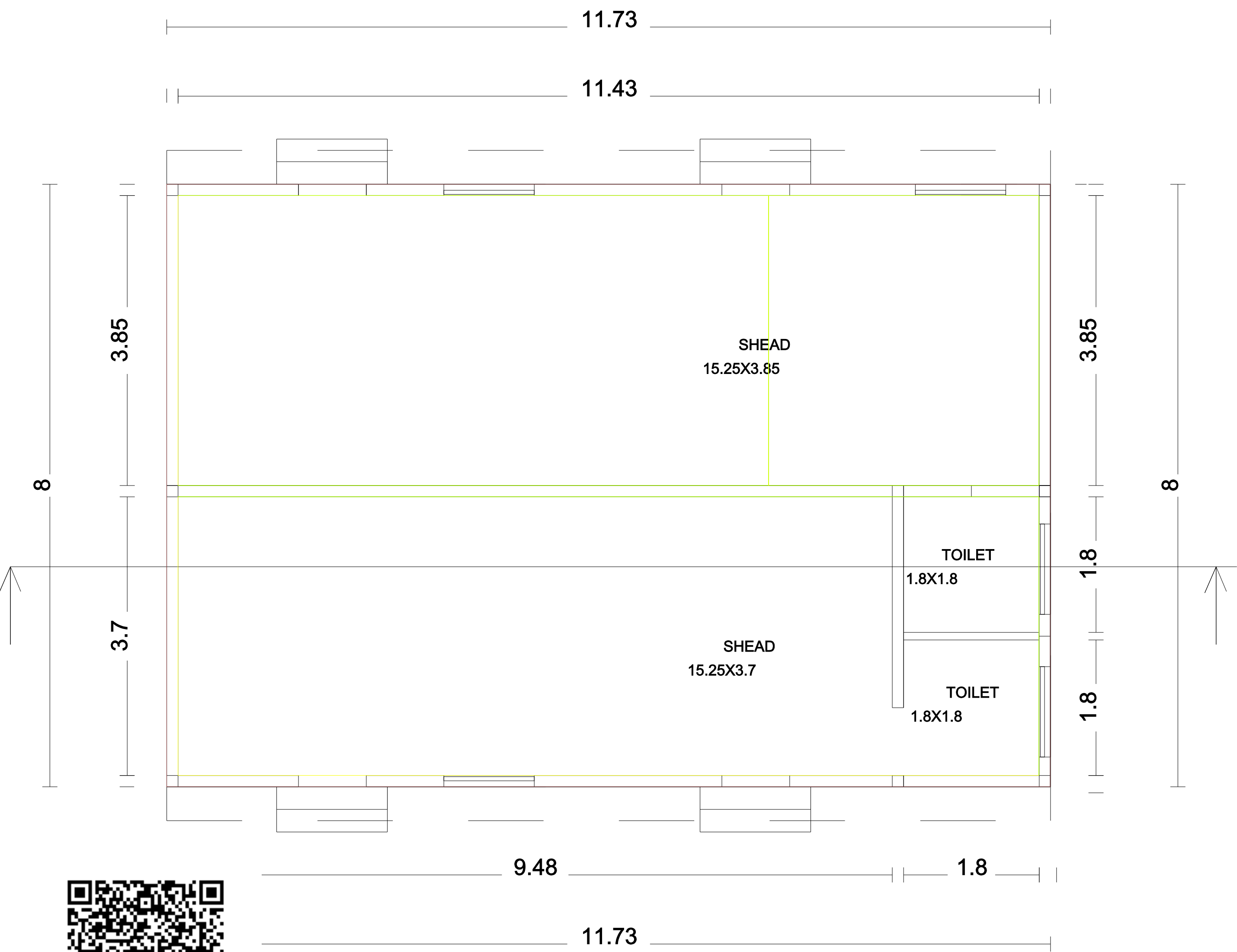
PLAN
