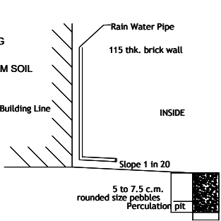
PERCOLATION PIT
