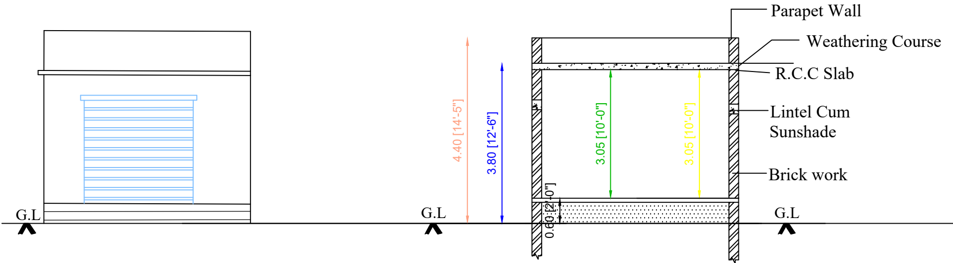
SECTION AB
