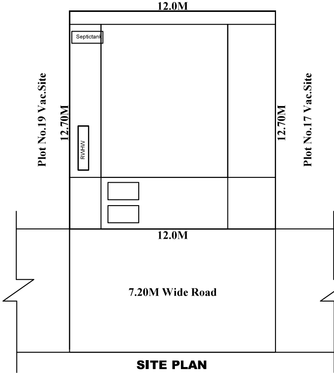
SITE PLAN
