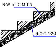
STAIRCASE
