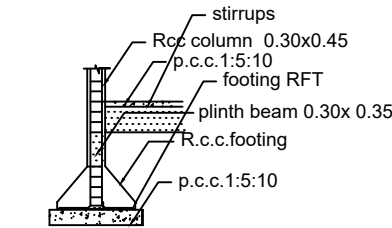
COLUMN DETAILS
