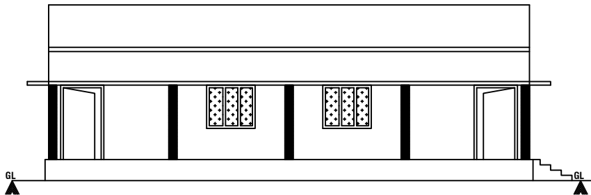
FRONT ELEVATION
