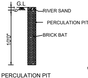
PERCULATION PIT
