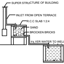
DETAILS OF FILTER BED & WELL NTS
