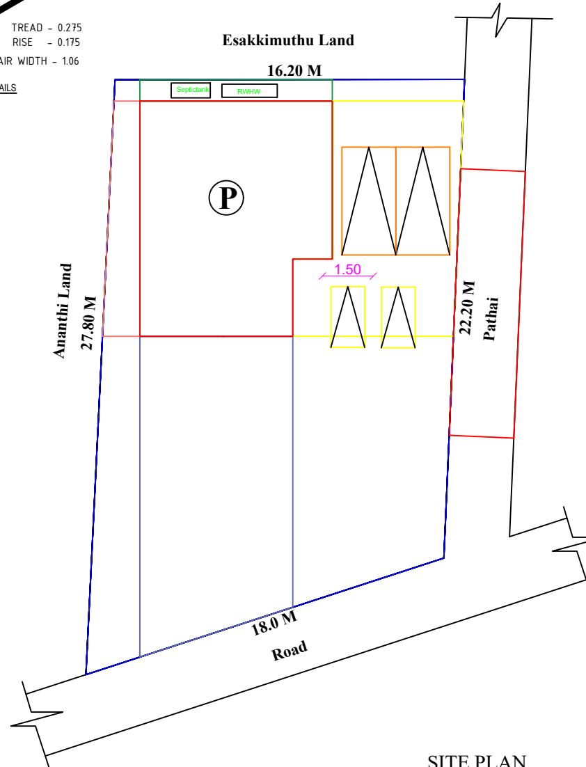
SITE PLAN
