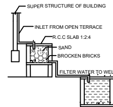
DETAILS OF FILTER BED & WELL
