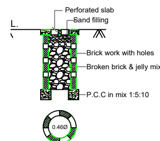
COLATION PIT FOR 30 Sq. m. (NOT FOR SCALE)
