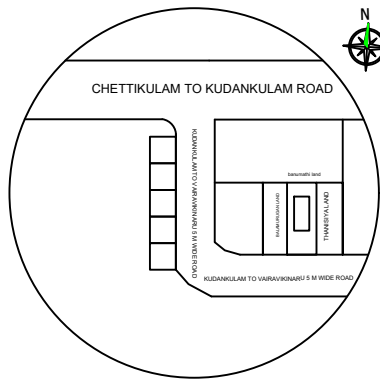
KEY PLAN 1:500 SCALE
