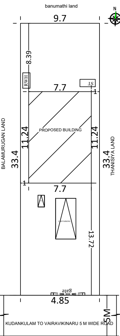
SITEPLAN 1:200 SCALE
