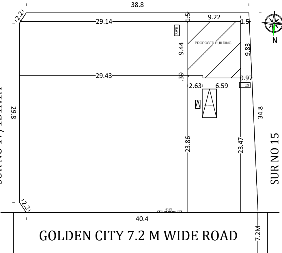
SITE PLAN 1:200 SCALE
