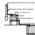
DETAILS OF FILTER BED & WELL NTS
