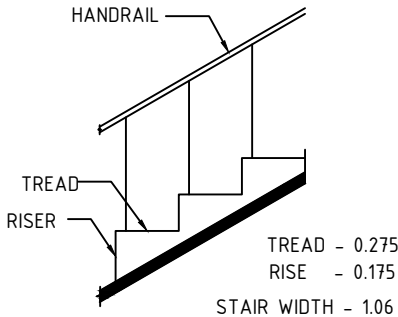
STAIRCASE DETAILS NTS
