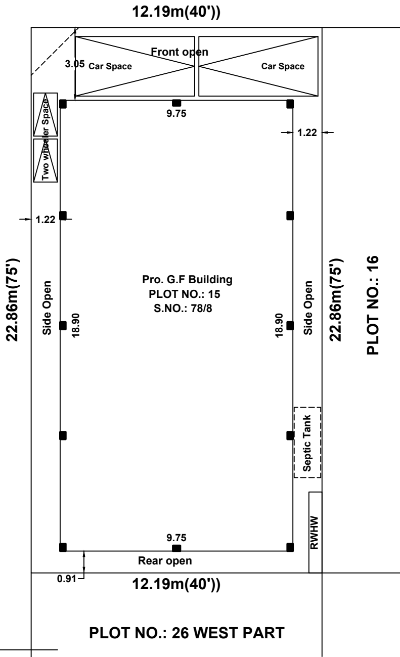
SITE PLAN
