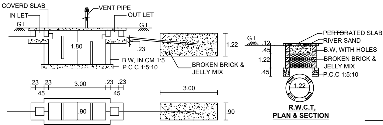
PLAN & SECTION OF SEPTIC TANK & TRENCH
