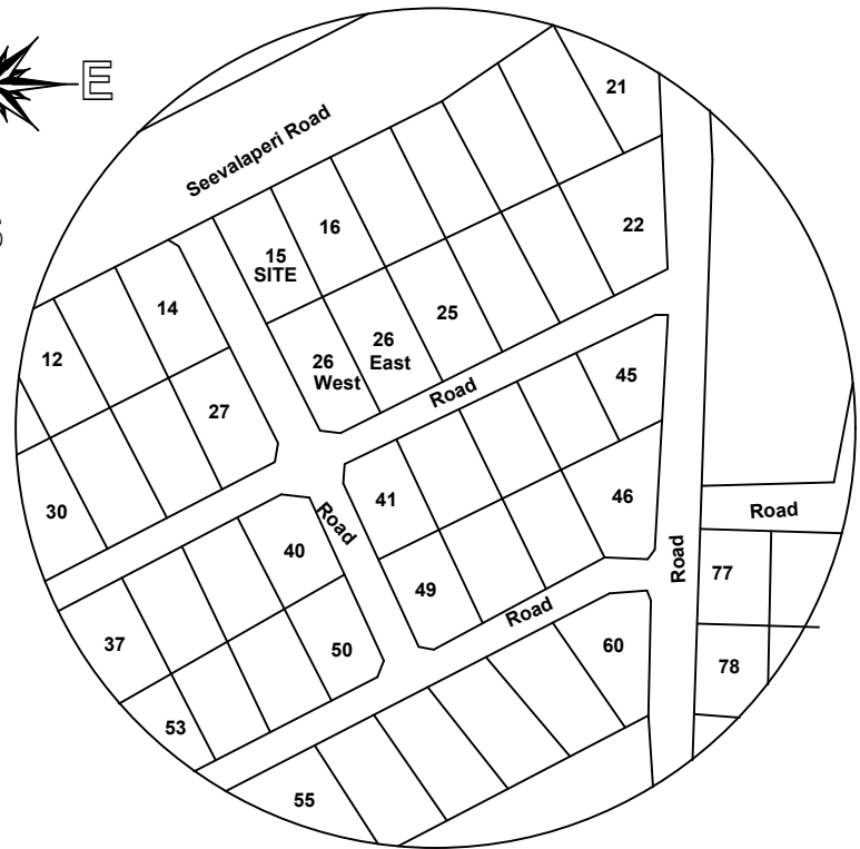
LAYOUT
