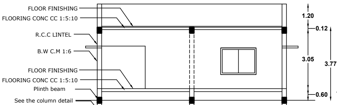
SECTION AT AA'
