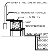
DETAILS OF FILTER BED & WELL
