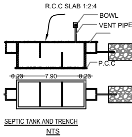
SEPTIC TANK AND TRENCH
