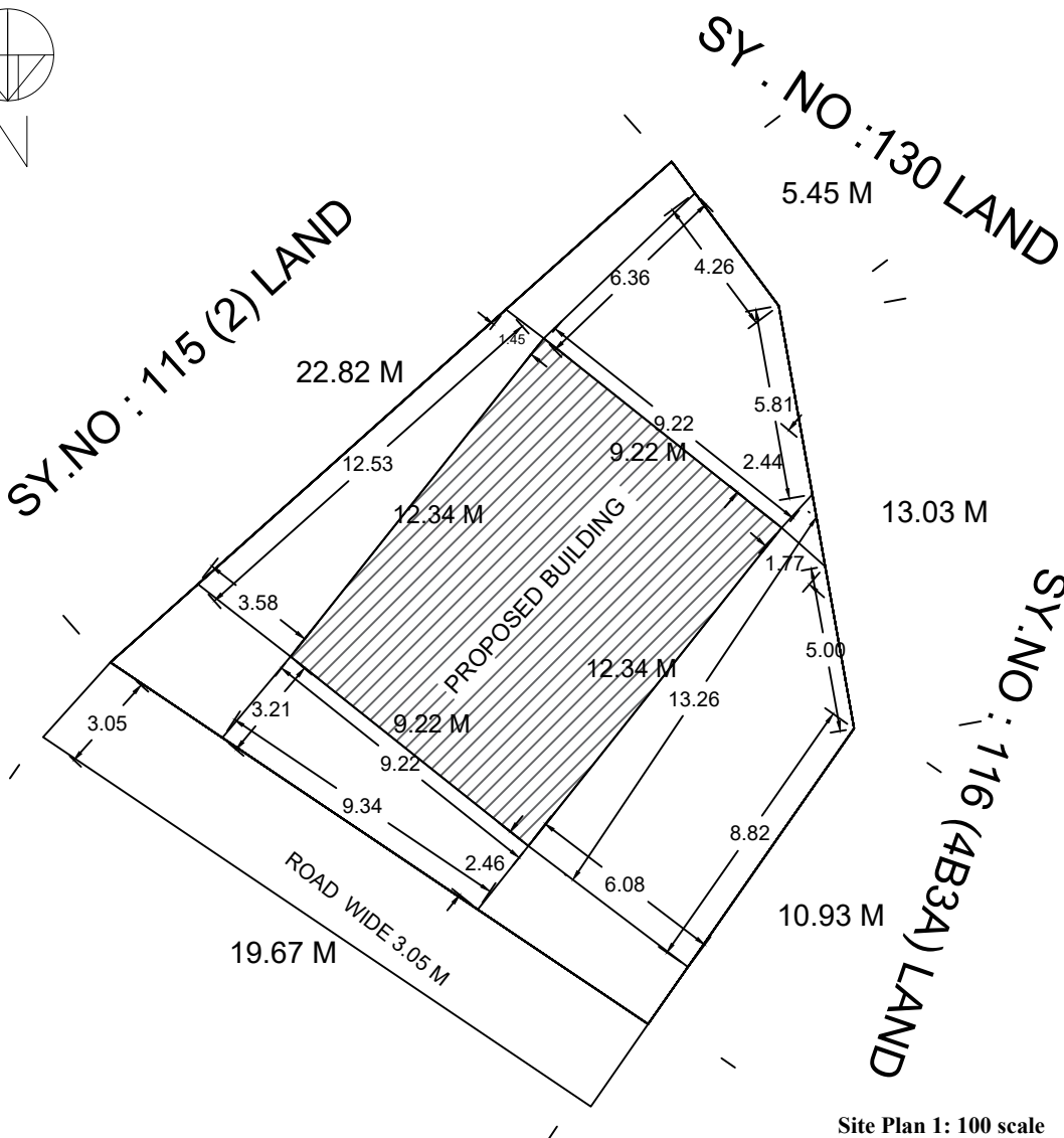
Site Plan 1: 100 scale
