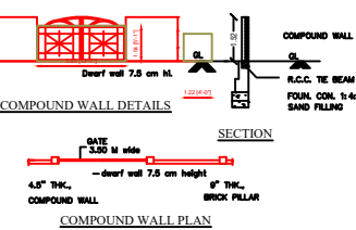
COMPOUND WALL PLAN
