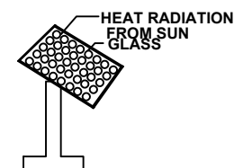
SOLAR SYSTEM
