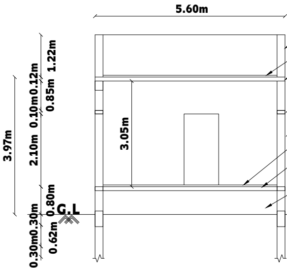
SECTION ON "G1G2"
