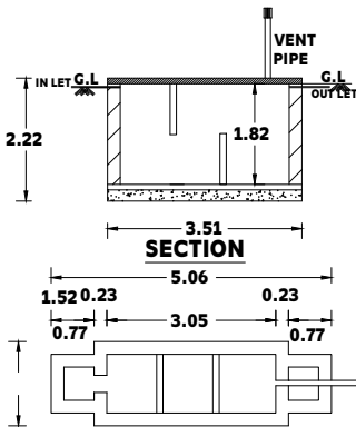
PLAN OF SEPTIC TANK AND TRENCH DETAILS
