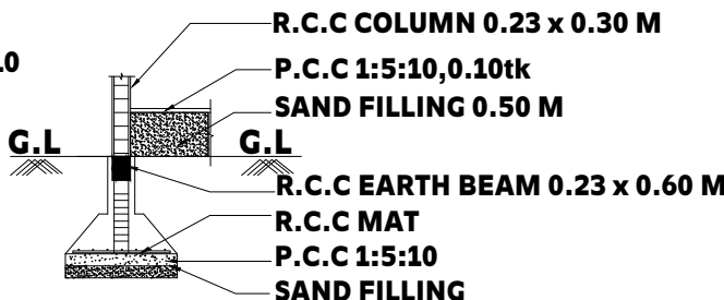
R.C.C COLUMN DETAILS
