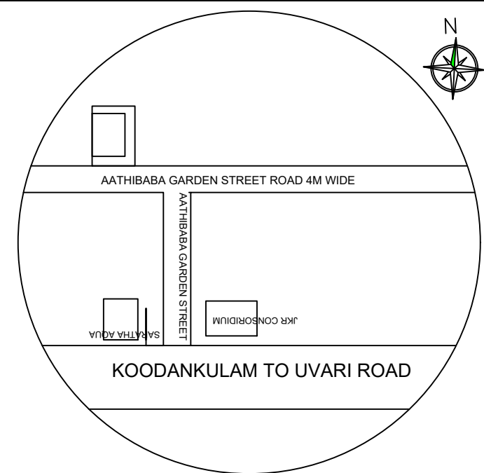
KEY PLAN 1:500 SCALE
