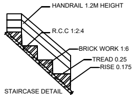
STAIRCASE DETAIL
