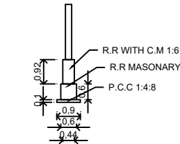
FOUNDATION
