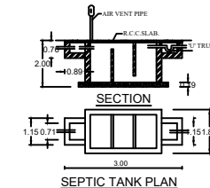
SEPTIC TANK PLAN
