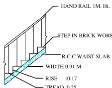
STAIR DETAIL
