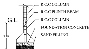
COLUMN DETAILS
