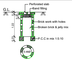
COLUMN DETAILS
