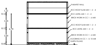
SECTION ON AB & ( HALF ELEVATION)
