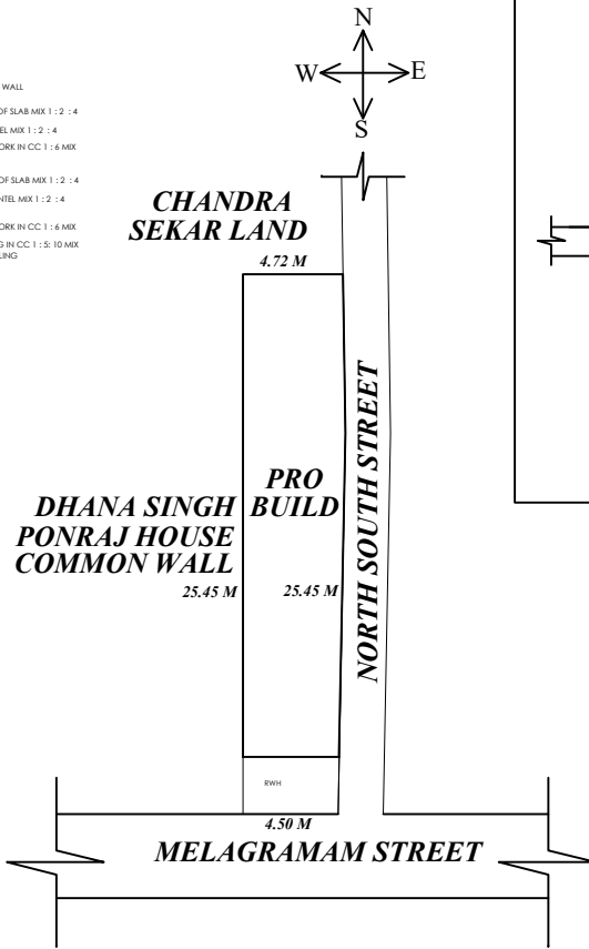
SITE PLAN
