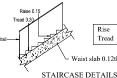
STAIRCASE DETAILS
