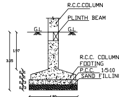
FOUNDATION DETAILS
