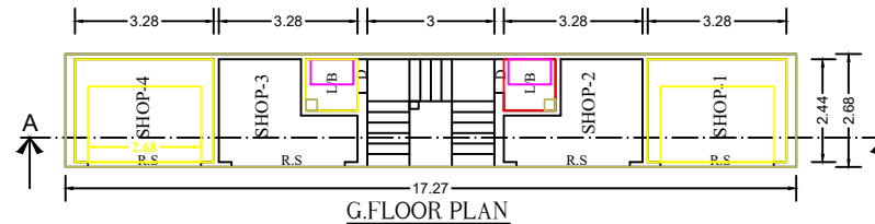
G.FLOOR PLAN
