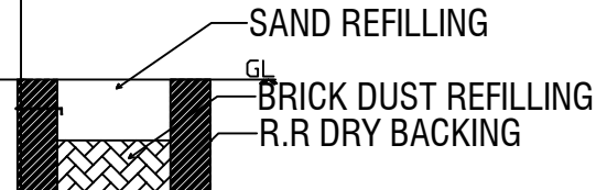
DETAILS OF RAIN WATER HARVESTING
