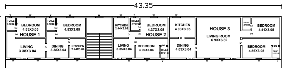
EXISTING GROUND FLOOR PLAN
