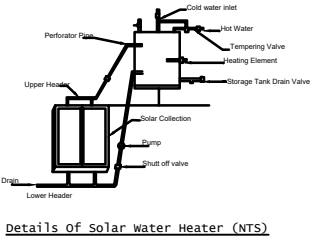
Details of Solar Water Heater (NTS)
