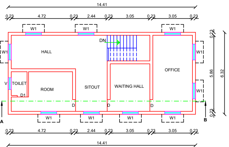
PRO. FIRST FLOOR PLAN
