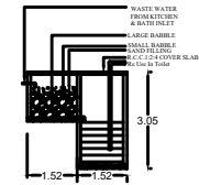
RECYCLING OF WASTE WATER FROM KITCHEN & BATHROOM
