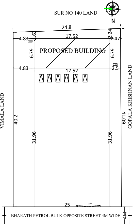
SITE PLAN 1:200 SCALE
