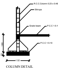
COLUMN DETAIL
