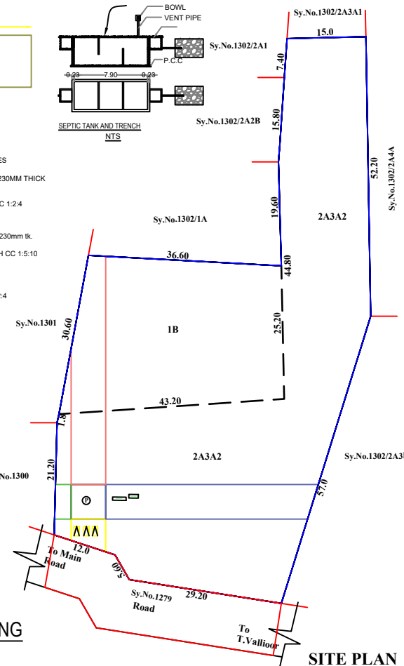
SITE PLAN
