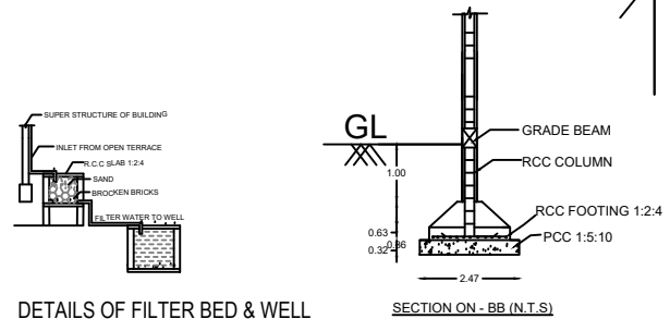
DETAILS OF FILTER BED & WELL NTS
